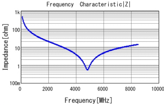
GCM1555C1H3R3CA16 |Z| DCOV, 25degC
