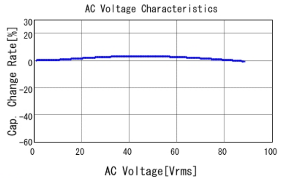
■ GC321AD72E103KX01 C-AC Voltage capchange, DC0V, 25.0d
