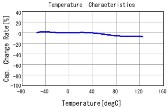
■ GCJ188R71H332KA01 C-Temp. capchange, DC0.0V, AC1.0Vrm
