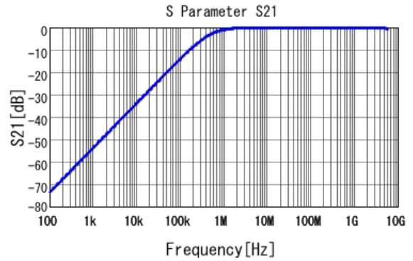
■ GCJ188R71H332KA01 S21 DC0V, 25degC
