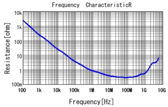
■ GCJ188R71H332KA01 R DCOV, 25degC
