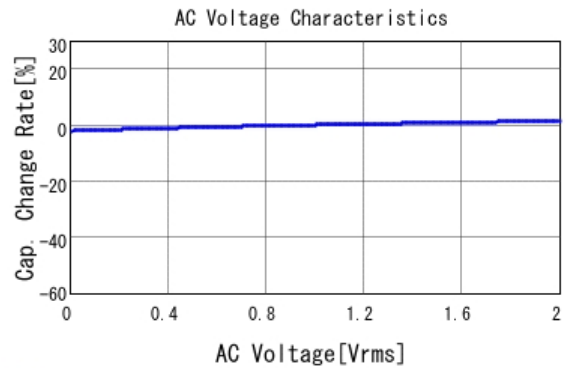
■ GCJ188R71H332KA01 C-AC Voltage capchange, DCOV, 25.0d
