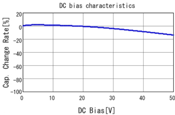
■ GCJ188R71H332KA01 C-DC bias capchange, 25.0degC, AC1.
