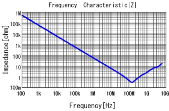
■ GCJ188R71H332KA01 |Z| DCOV, 25degC
