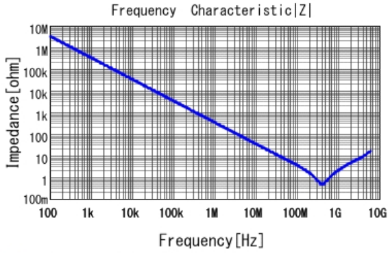
GCM155R71H471KA37 |Z| DCOV, 25degC
