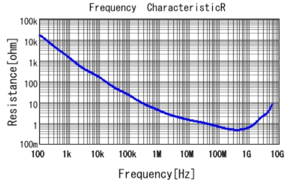
GCM155R71H471KA37 R DCOV, 25degC
