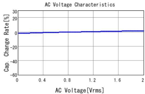
GCM155R71H471KA37 C-AC Voltage capchange, DCOV, 25.0d
