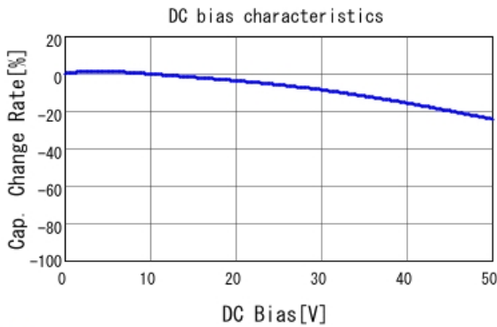
GCM155R71H471KA37 C-DC bias capchange, 25.0degC, AC1.
