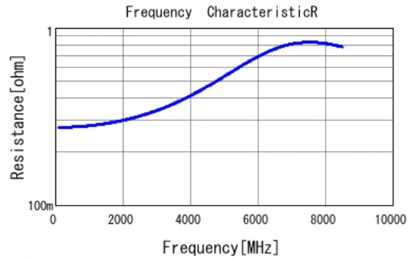
■ GCM1555C1H3R0CA16 R DCOV, 25degC
