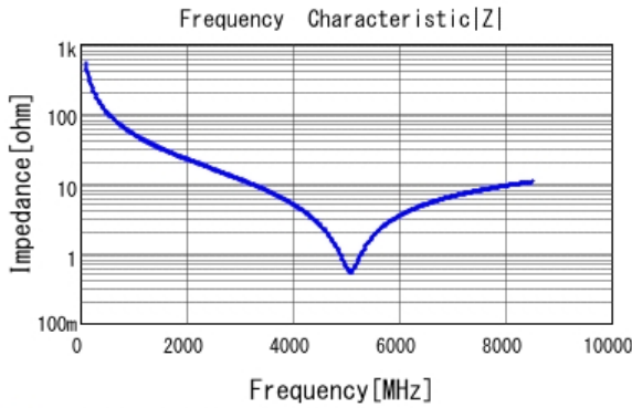
■ GCM1555C1H3R0CA16 |Z| DCOV, 25degC
