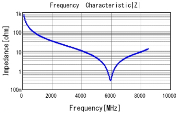
■ GJM1555C1H2R2BB01 |Z| DC0V, 25degC
