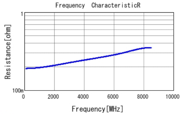
■ GJM1555C1H2R2BB01 R DC0V, 25degC
