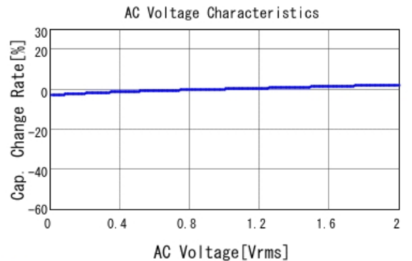
■ GRM155R72A222KA01 C-AC Voltage capchange, DCOV, 25.0d
