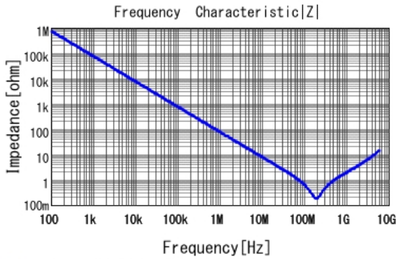
■ GRM155R72A222KA01 |Z| DCOV, 25degC
