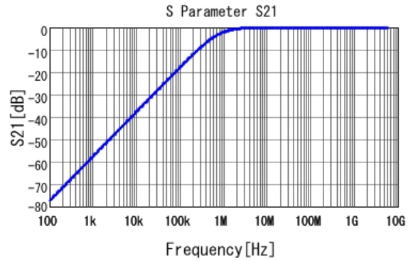
■ GRM155R72A222KA01 S21 DC0V, 25degC
