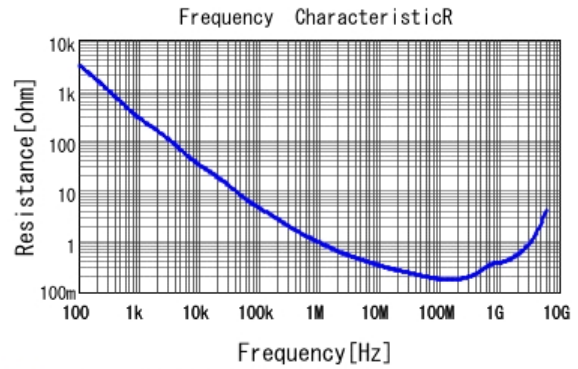
■ GRM155R72A222KA01 R DCOV, 25degC
