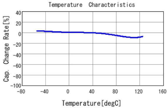
■ GRM155R72A222KA01 C-Temp. capchange, DC0.0V, AC1.0V rm
