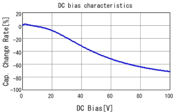
■ GRM155R72A222KA01 C-DC bias capchange, 25.0degC, AC1.
