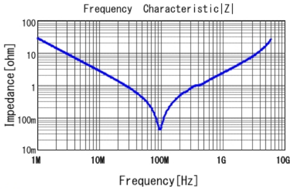
■ GRM1857U1A562JA44 |Z| DCOV, 25degC
