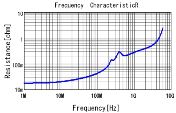
■ GRM1857U1A562JA44 R DCOV, 25degC
