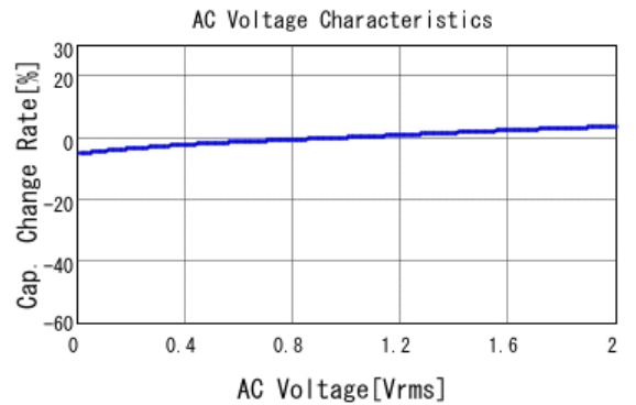
■ GRM155R62A104KE14 C-AC Voltage capchange, DCOV, 25.0d
