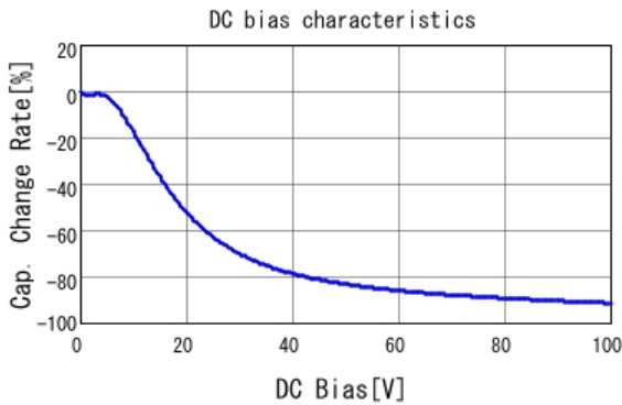
■ GRM155R62A104KE14 C-DC bias capchange, 25.0degC, AC1.
