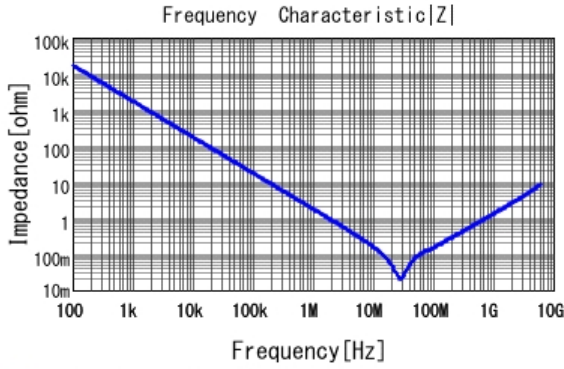
■ GRM155R62A104KE14 |Z| DCOV, 25degC
