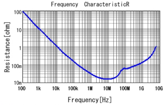
■ GRM155R62A104KE14 R DCOV, 25degC
