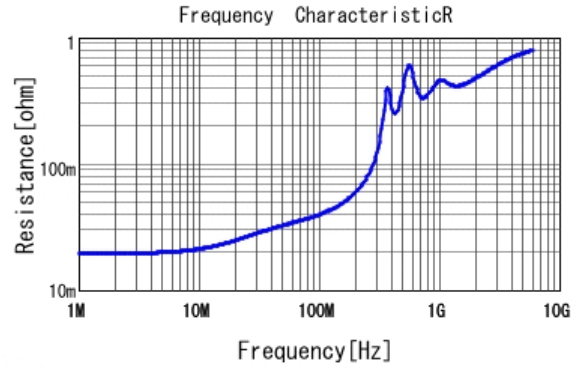
■ GRM1885C1H152JA01 R DCOV, 25degC
