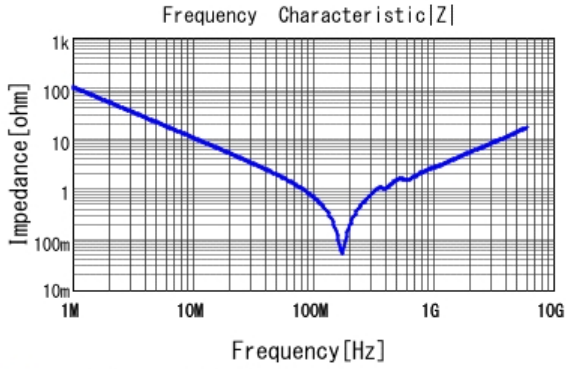
■ GRM1885C1H152JA01 |Z| DCOV, 25degC
