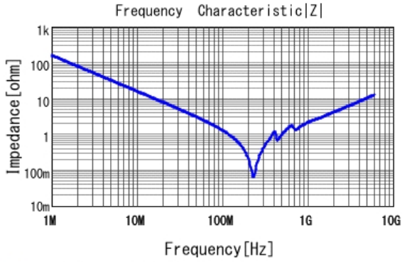
■ GRM1885C1H102JA01 |Z| DCOV, 25degC
