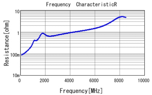
■ GRM1555C1H271JA01 R DCOV, 25degC
