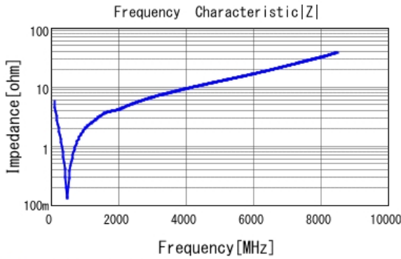
■ GRM1555C1H271JA01 |Z| DCOV, 25degC
