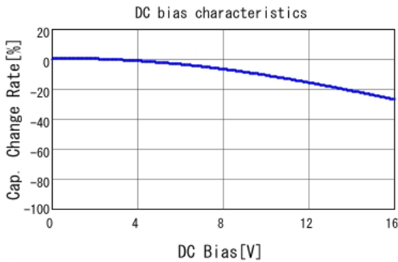
GCM155R71C333KA37 C-DC bias capchange, 25.0degC, AC1.
