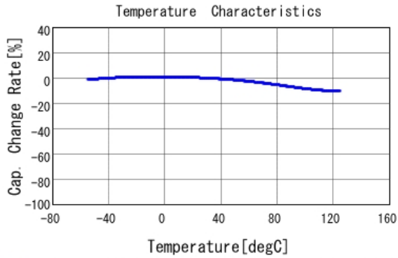
■ GCM155R71C333KA37 C-Temp. capchange, DC0.0V, AC1.0V rm
