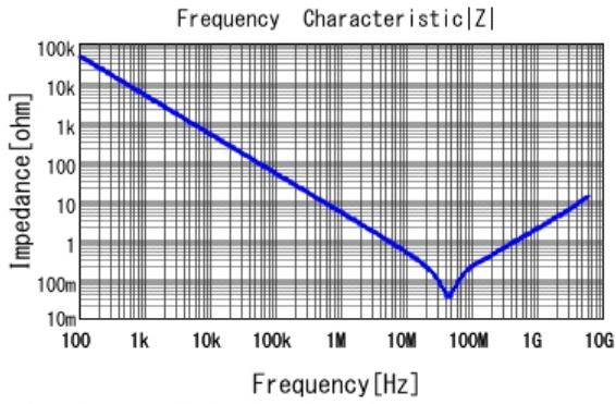
GCM155R71C333KA37 |Z| DCOV, 25degC
