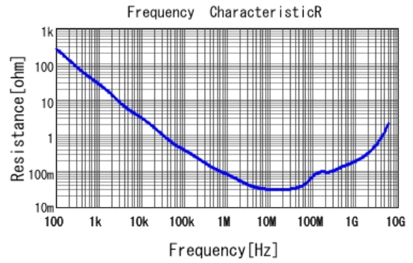
GCM155R71C333KA37 R DCOV, 25degC
