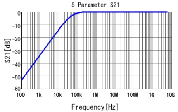
■ GCM155R71C333KA37 S21 DC0V, 25degC
