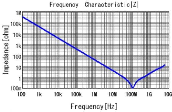
■ GCD188R72A472KA01 |Z| DCOV, 25degC
