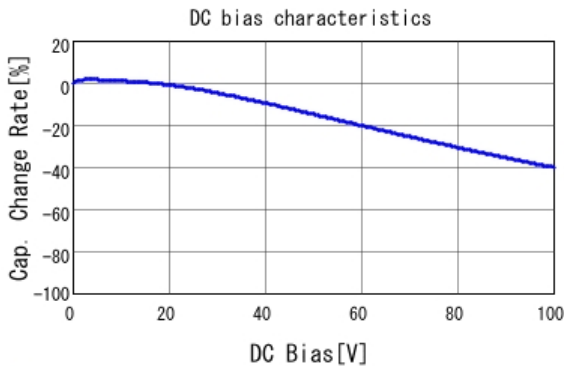
■ GCD188R72A472KA01 C-DC bias capchange, 25.0degC, AC1.
