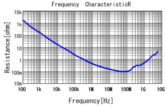
■ GCD188R72A472KA01 R DCOV, 25degC
