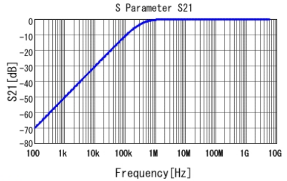
■ GCD188R72A472KA01 S21 DC0V, 25degC
