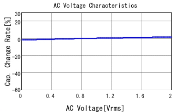
■ GCD188R72A472KA01 C-AC Voltage capchange, DCOV, 25.0d
