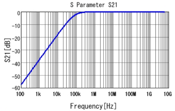
■ GCE188R71H223KA01 S21 DC0V, 25degC
