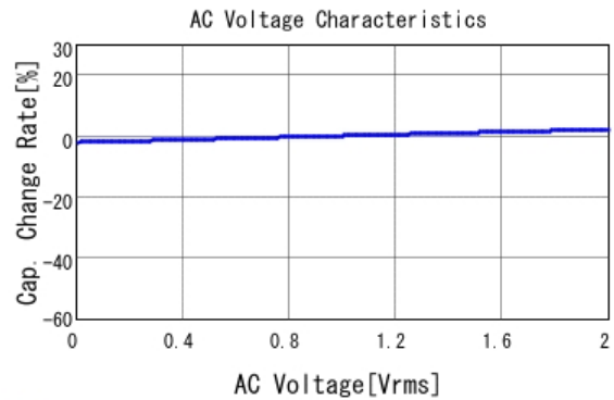
■ GCE188R71H223KA01 C-AC Voltage capchange, DCOV, 25.0d
