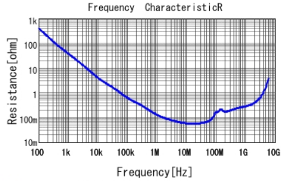
■ GCE188R71H223KA01 R DCOV, 25degC
