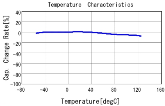
■ GCE188R71H223KA01 C-Temp. capchange, DC0.0V, AC1.0Vrm
