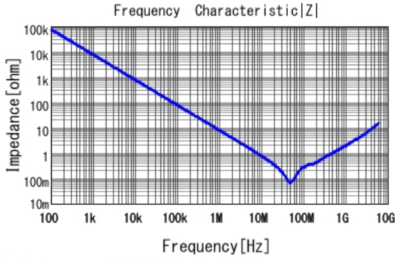
■ GCE188R71H223KA01 |Z| DCOV, 25degC
