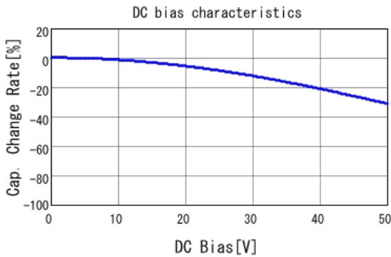
■ GCE188R71H223KA01 C-DC bias capchange, 25.0degC, AC1.
