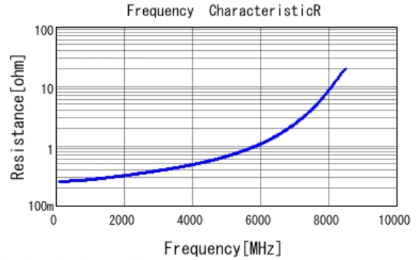
■ GCM1555C1H3R9BA16 R DCOV, 25degC
