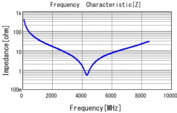
■ GCM1555C1H3R9BA16 |Z| DCOV, 25degC
