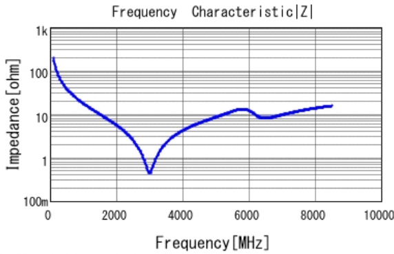
■ GCM1555C1H8R0DA16 |Z| DCOV, 25degC
