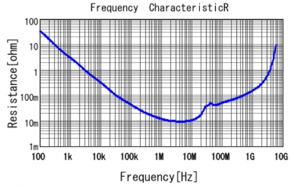
■ GCM188R71H224KA64 R DC0V, 25degC
