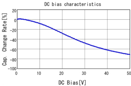
■ GCM188R71H224KA64 C-DC bias capchange, 25.0degC, AC1.
