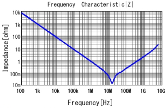
■ GCM188R71H224KA64 |Z| DC0V, 25degC
