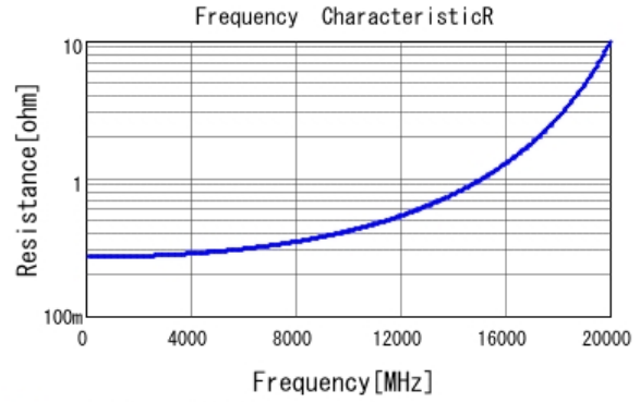
■ GJM1555C1HR80BB01 R DCOV, 25degC
