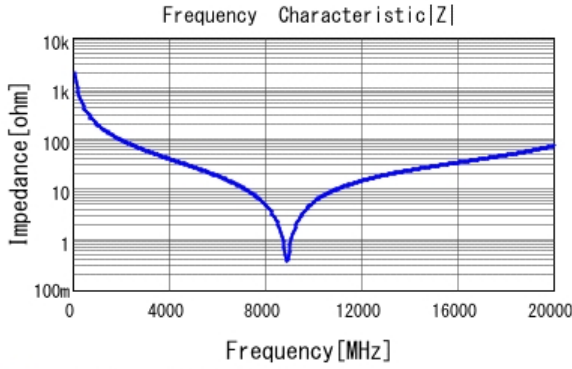
■ GJM1555C1HR80BB01 |Z| DCOV, 25degC
