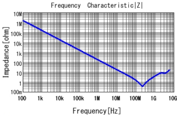
■ GCE188R72A102KA01 |Z| DCOV, 25degC
