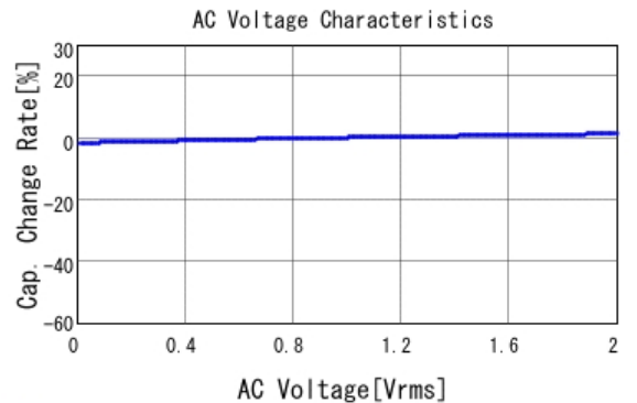
■ GCE188R72A102KA01 C-AC Voltage capchange, DCOV, 25.0d
