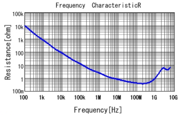
■ GCE188R72A102KA01 R DCOV, 25degC
