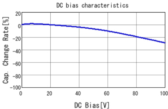
■ GCE188R72A102KA01 C-DC bias capchange, 25.0degC, AC1.
