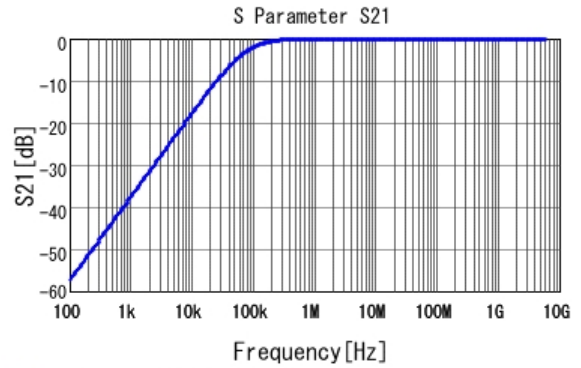
■ GCM155R71H223KA55 S21 DC0V, 25degC
