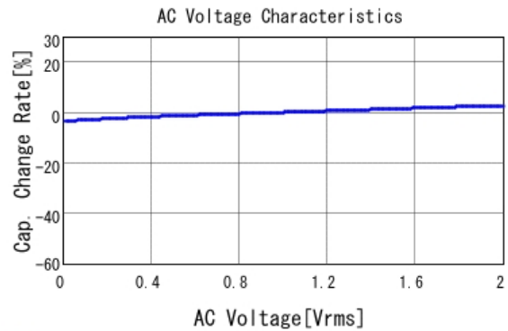
GCM155R71H223KA55 C-AC Voltage capchange, DC0V, 25.0d
