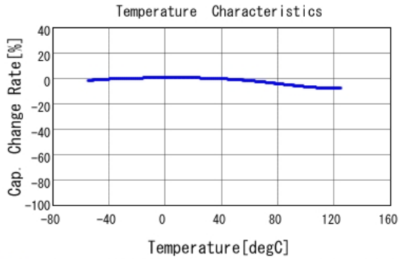
■ GCM155R71H223KA55 C-Temp. capchange, DC0.0V, AC1.0V rm
