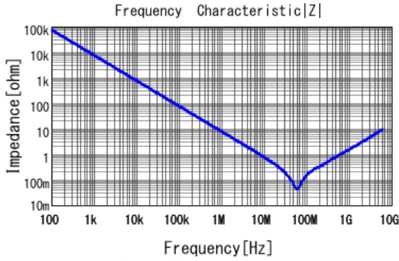
GCM155R71H223KA55 |Z| DC0V, 25degC
