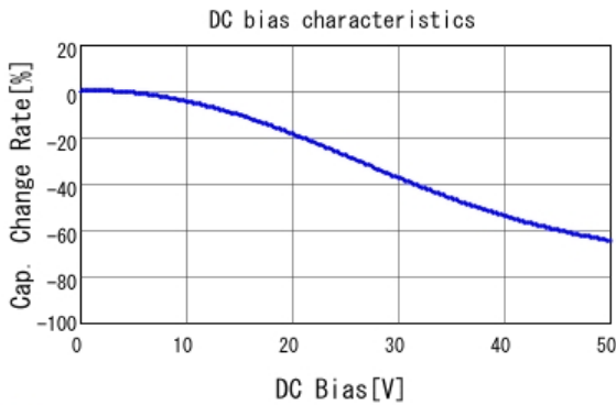
GCM155R71H223KA55 C-DC bias capchange, 25.0degC, AC1.
