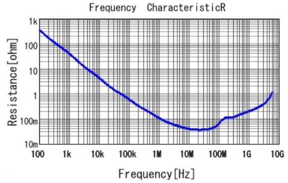
GCM155R71H223KA55 R DC0V, 25degC
