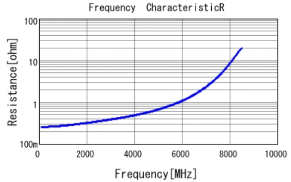
GCM1555C1H3R9CA16 R DCOV, 25degC
