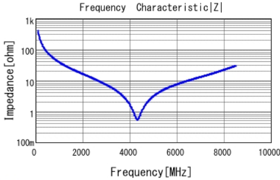
GCM1555C1H3R9CA16 |Z| DCOV, 25degC
