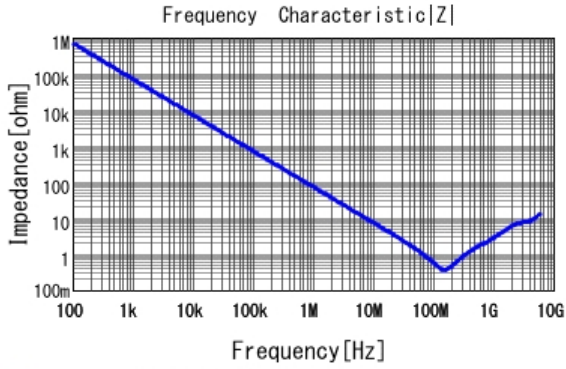
■ GCJ188R72A222KA01 |Z| DCOV, 25degC
