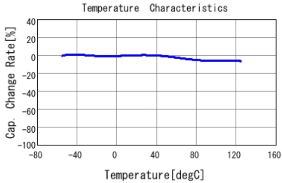
■ GCJ188R72A222KA01 C-Temp. capchange, DC0.0V, AC1.0Vrm
