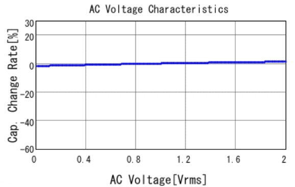
■ GCJ188R72A222KA01 C-AC Voltage capchange, DCOV, 25.0d
