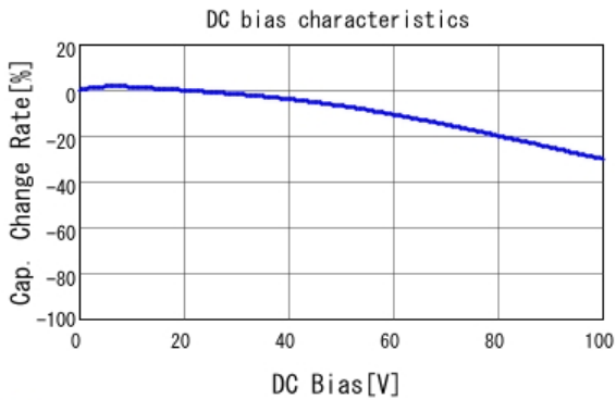
■ GCJ188R72A222KA01 C-DC bias capchange, 25.0degC, AC1.
