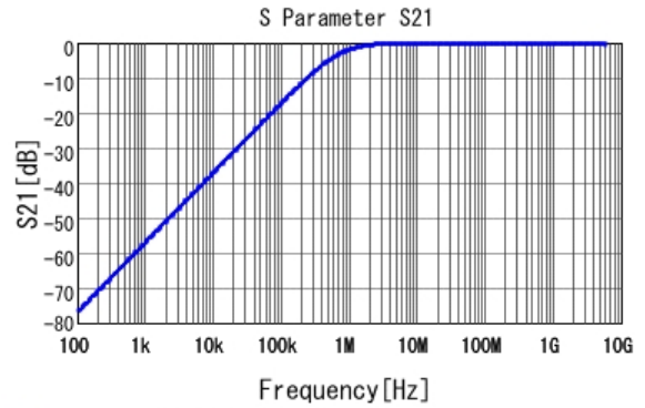
■ GCJ188R72A222KA01 S21 DC0V, 25degC
