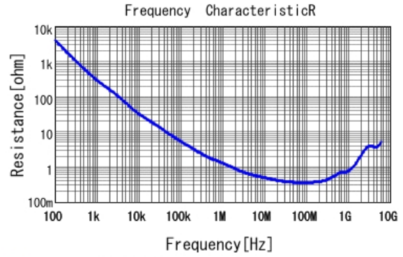
■ GCJ188R72A222KA01 R DCOV, 25degC
