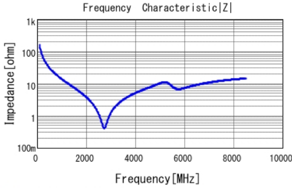
■ GCM1555C1H100GA16 |Z| DCOV, 25degC
