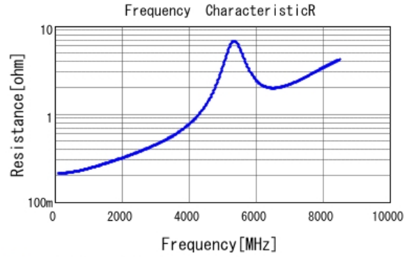
■ GCM1555C1H100GA16 R DCOV, 25degC
