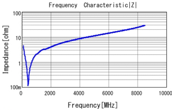
■ GCM1555C1H331JA16 |Z| DCOV, 25degC
