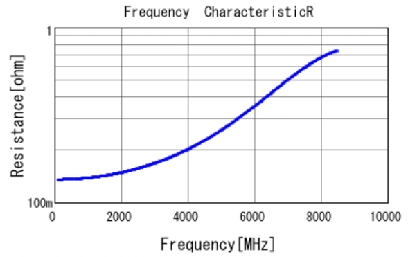
■ GJM1555C1H3R0CB01 R DCOV, 25degC
