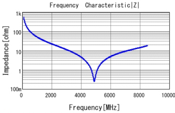
■ GJM1555C1H3R0CB01 |Z| DCOV, 25degC
