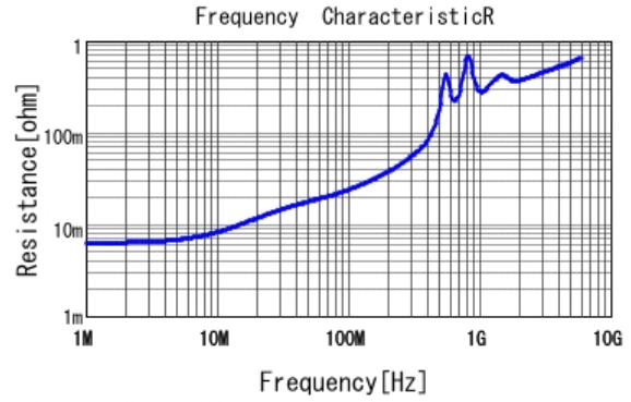
GCM1555C1H102FA16 R DCOV, 25degC
