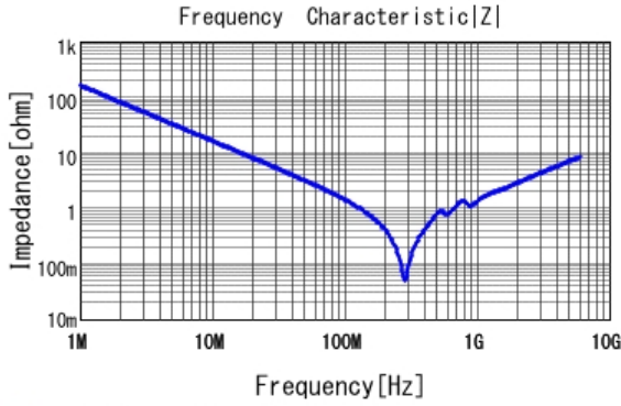
GCM1555C1H102FA16 |Z| DCOV, 25degC
