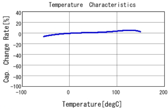
■ GCJ188R92A102KA01 C-Temp. capchange, DC0.0V, AC1.0Vrm
