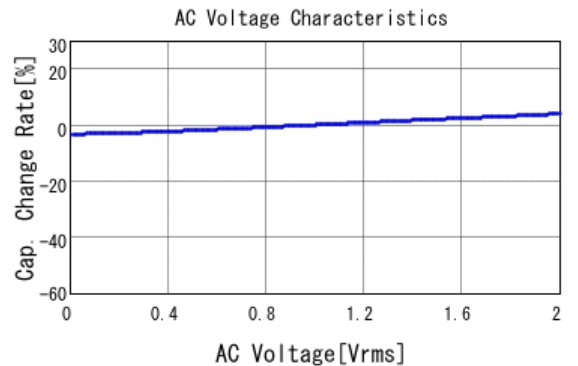
■ GCJ188R92A102KA01 C-AC Voltage capchange, DCOV, 25.0d
