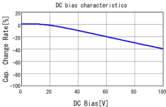
■ GCJ188R92A102KA01 C-DC bias capchange, 25.0degC, AC1.
