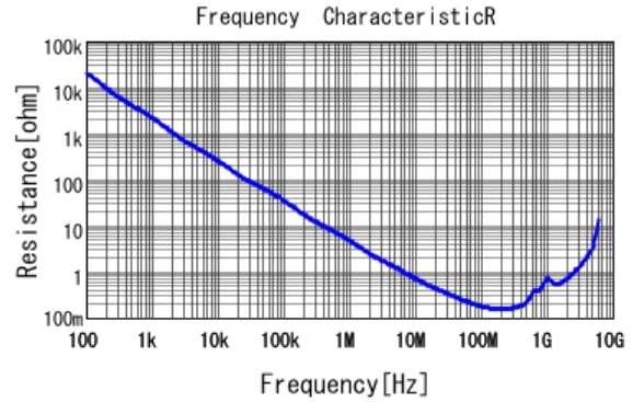
■ GCJ188R92A102KA01 R DCOV, 25degC
