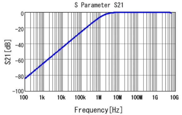
■ GCJ188R92A102KA01 S21 DC0V, 25degC
