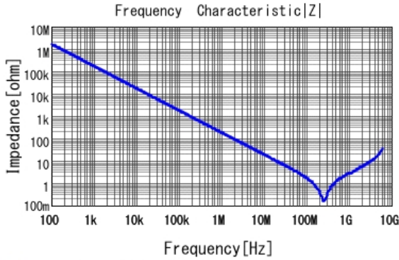
■ GCJ188R92A102KA01 |Z| DCOV, 25degC
