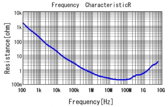
■ GCJ188R72A472KA01 R DCOV, 25degC
