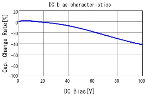
■ GCJ188R72A472KA01 C-DC bias capchange, 25.0degC, AC1.
