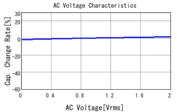
■ GCJ188R72A472KA01 C-AC Voltage capchange, DCOV, 25.0d
