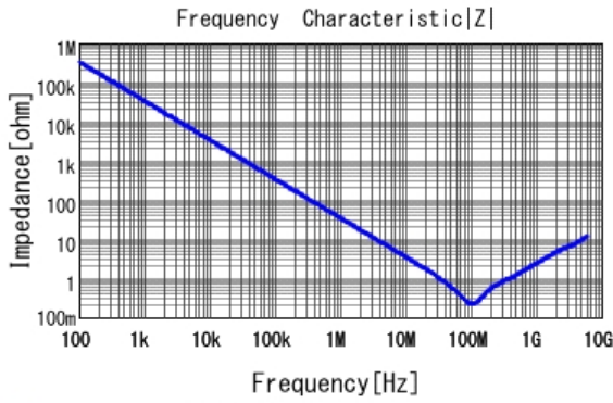
■ GCJ188R72A472KA01 |Z| DCOV, 25degC
