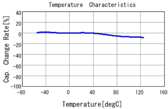
■ GCJ188R72A472KA01 C-Temp. capchange, DC0.0V, AC1.0Vrm
