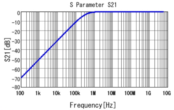
■ GCJ188R72A472KA01 S21 DC0V, 25degC
