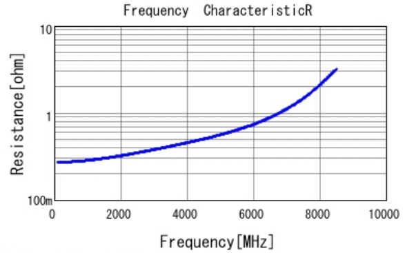
■ GCM1555C1H3R3BA16 R DCOV, 25degC
