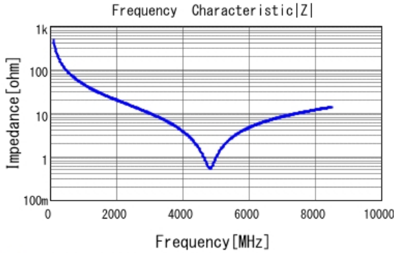
■ GCM1555C1H3R3BA16 |Z| DCOV, 25degC
