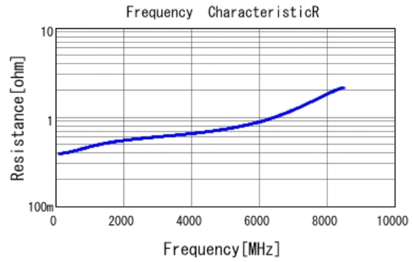
■ GCM1555C1H1R5JA16 R DCOV, 25degC
