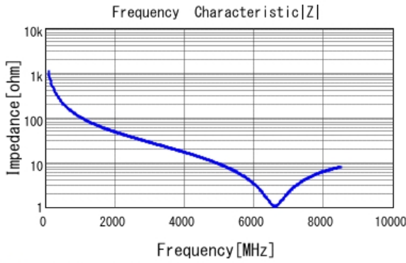
■ GCM1555C1H1R5JA16 |Z| DCOV, 25degC
