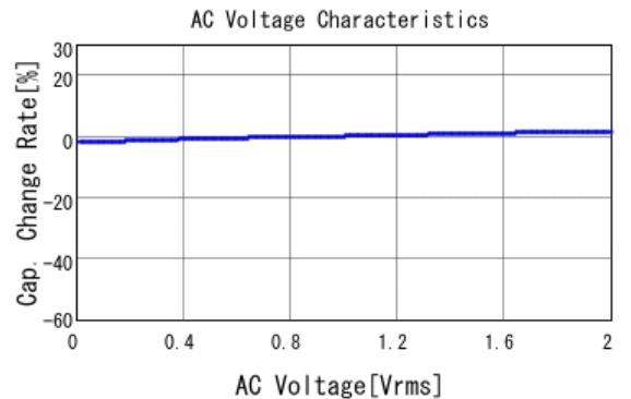
GCM155R72A331KA37 C-AC Voltage capchange, DCOV, 25.0d
