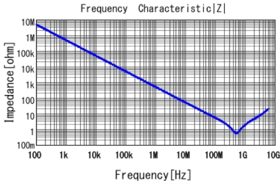
GCM155R72A331KA37 |Z| DCOV, 25degC
