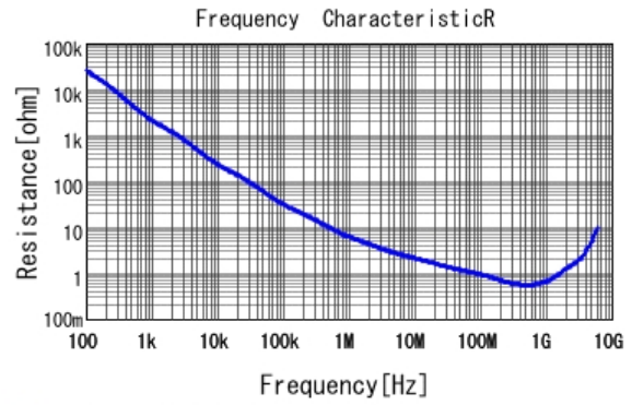
GCM155R72A331KA37 R DCOV, 25degC
