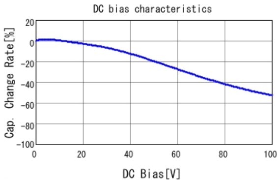
GCM155R72A331KA37 C-DC bias capchange, 25.0degC, AC1.
