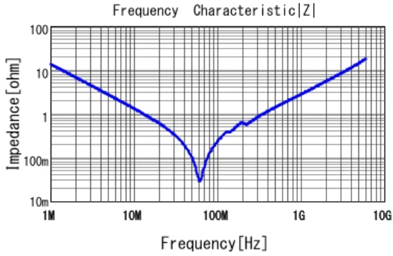
■ GRM1887U1A123JA01 |Z| DCOV, 25degC
