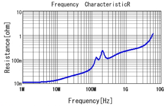
■ GRM1887U1A123JA01 R DCOV, 25degC
