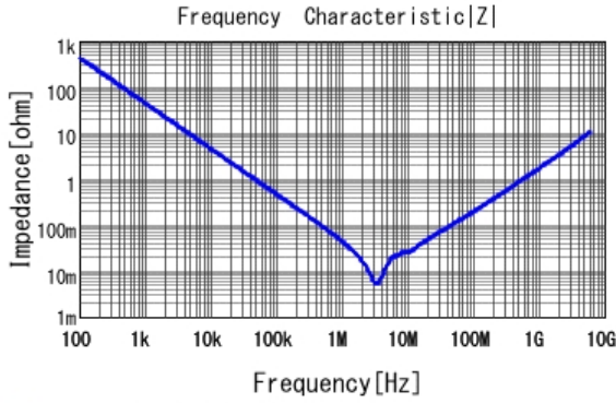
■ GRT188R6YA475KE13 |Z| DCOV, 25degC
