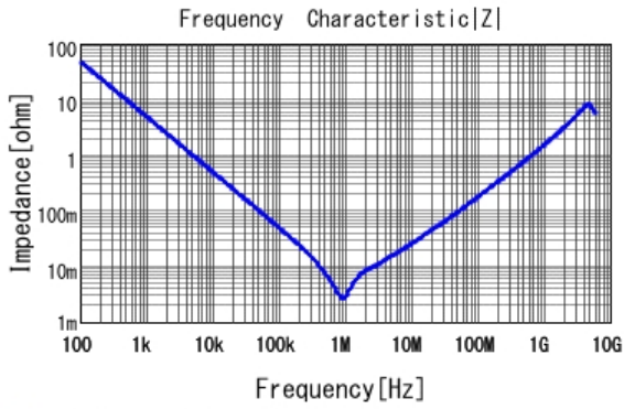
■ GRM219R60J476ME44 |Z| DCOV, 25degC
