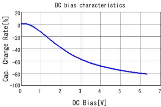
■ GRM219R60J476ME44 C-DC bias capchange, 25.0degC, AC0.
