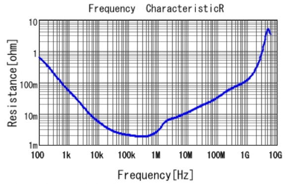
■ GRM219R60J476ME44 R DCOV, 25degC
