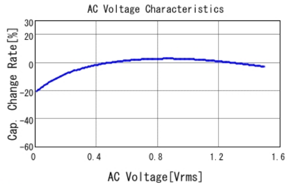
■ GRM219R60J476ME44 C-AC Voltage capchange, DCOV, 25.0d
