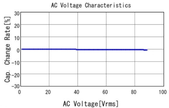
■ GRM21A7U2E331JW31 C-AC Voltage capchange, DCOV, 25.0d
