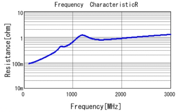
■ GRM21A7U2E331JW31 R DCOV, 25degC
