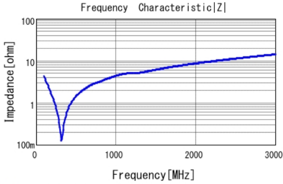
■ GRM21A7U2E331JW31 |Z| DCOV, 25degC
