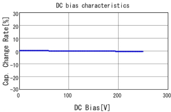
■ GRM21A7U2E121JW31 C-DC bias capchange, 25.0degC, AC1V
