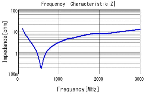
■ GRM21A7U2E121JW31 |Z| DCOV, 25degC
