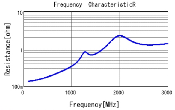
■ GRM21A7U2E121JW31 R DCOV, 25degC
