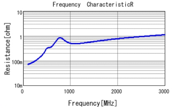
■ GRM21A7U2E681JW31 R DCOV, 25degC
