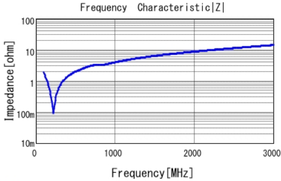
■ GRM21A7U2E681JW31 |Z| DCOV, 25degC
