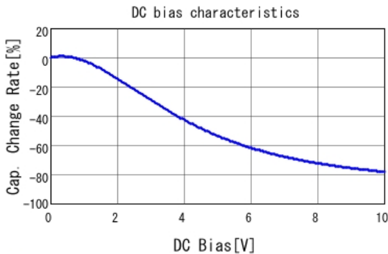
■ GRT21BC81A226ME13 C-DC bias capchange, 25.0degC, AC0.
