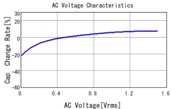
■ GRT21BC81A226ME13 C-AC Voltage capchange, DCOV, 25.0d
