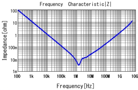
■ GRT21BC81A226ME13 |Z| DCOV, 25degC
