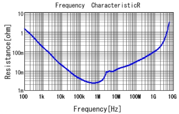
■ GRT21BC81A226ME13 R DCOV, 25degC
