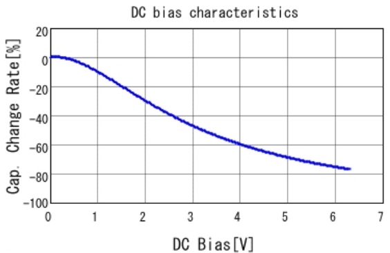
■ GRT188R60J106ME13 C-DC bias capchange, 25.0degC, AC0.
