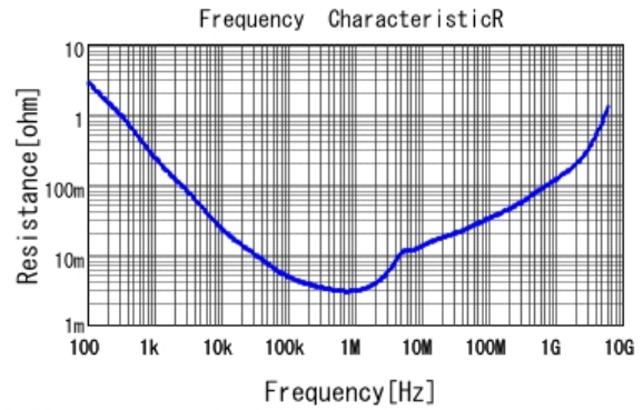
■ GRT188R60J106ME13 R DCOV, 25degC
