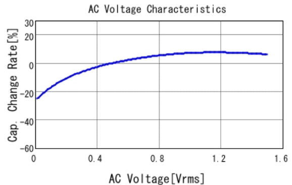
■ GRT188R60J106ME13 C-AC Voltage capchange, DCOV, 25.0d
