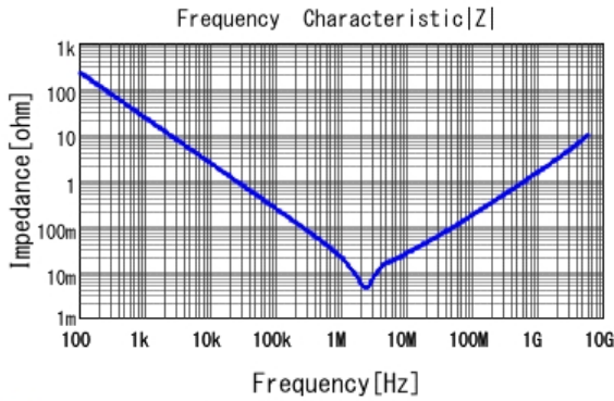
■ GRT188R60J106ME13 |Z| DCOV, 25degC
