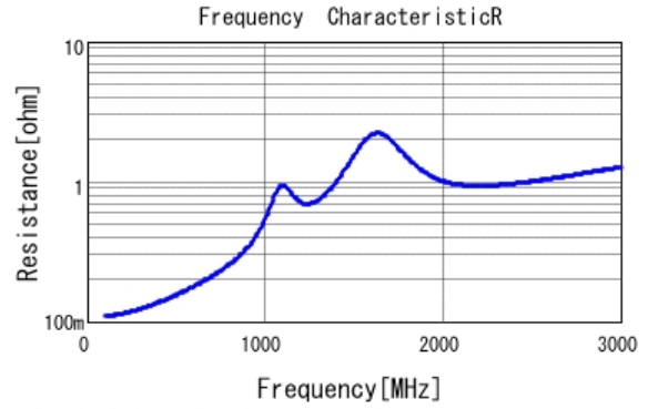
■ GRM21A7U2E151JW31 R DCOV, 25degC
