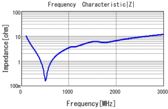
■ GRM21A7U2E151JW31 |Z| DCOV, 25degC
