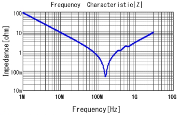
■ GRM21A7U2E182JW31 |Z| DCOV, 25degC
