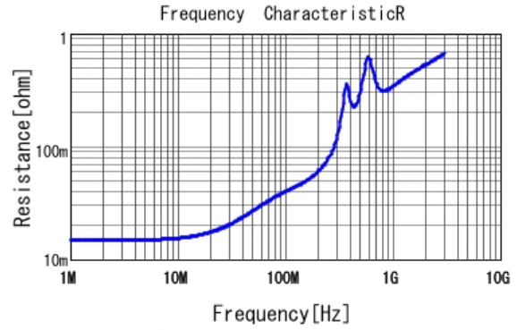
■ GRM21A7U2E182JW31 R DCOV, 25degC
