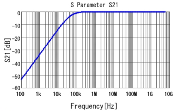
■ GCM155R71E333KA55 S21 DC0V, 25degC
