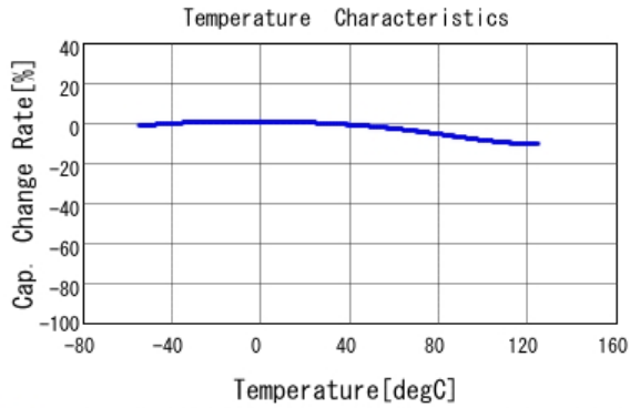
■ GCM155R71E333KA55 C-Temp. capchange, DC0.0V, AC1.0V rm
