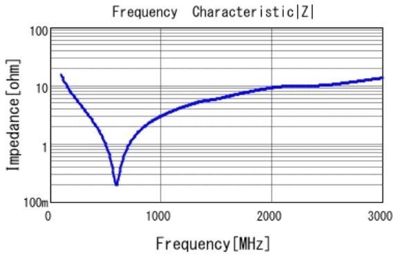
■ GRM21A7U2E101JW31 |Z| DCOV, 25degC
