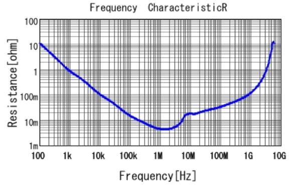
■ GRT21BC8YA475KE13 R DCOV, 25degC
