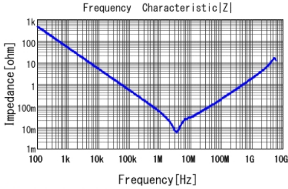
■ GRT21BC8YA475KE13 |Z| DCOV, 25degC
