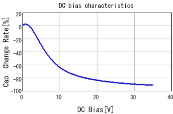
■ GRT21BC8YA475KE13 C-DC bias capchange, 25.0degC, AC1.
