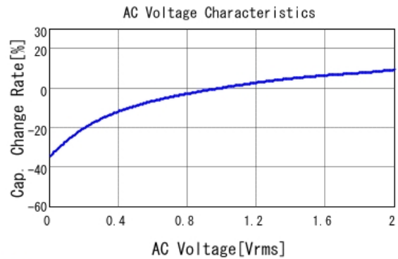
■ GRT21BC8YA475KE13 C-AC Voltage capchange, DCOV, 25.0d
