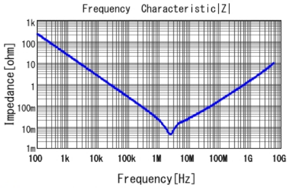
■ GRT188C80G106ME13 |Z| DCOV, 25degC
