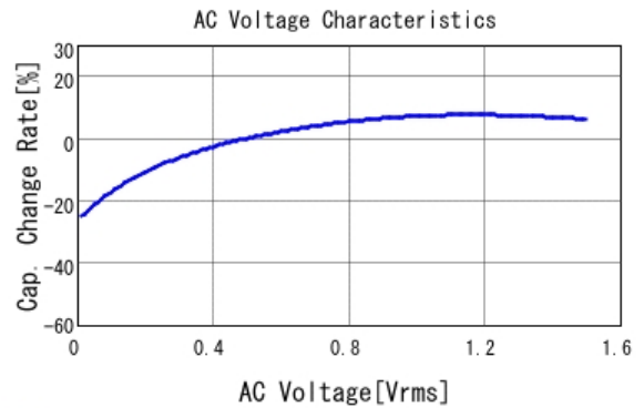
■ GRT188C80G106ME13 C-AC Voltage capchange, DCOV, 25.0d
