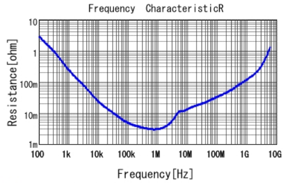
■ GRT188C80G106ME13 R DCOV, 25degC
