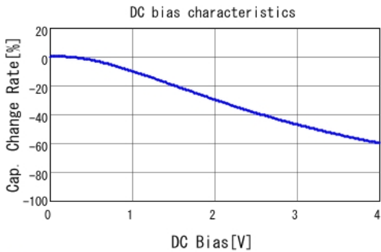
■ GRT188C80G106ME13 C-DC bias capchange, 25.0degC, AC0.
