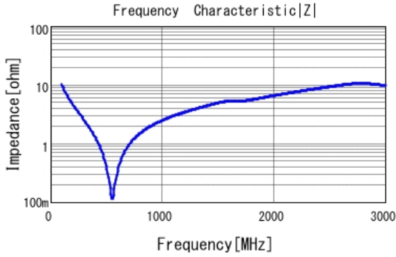
■ GRM21A5C2E151JW01 |Z| DC0V, 25degC
