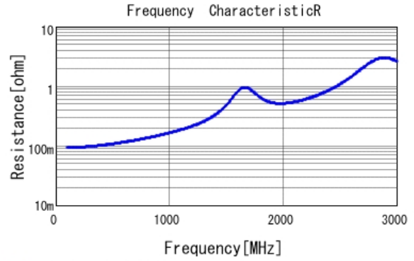
■ GRM21A5C2E151JW01 R DC0V, 25degC
