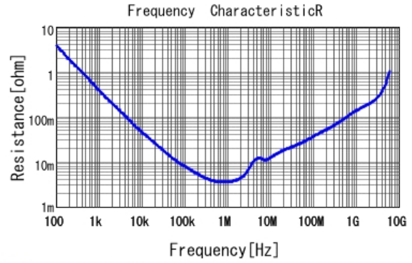
■ GRM188R61C106MAAL R DCOV, 25degC
