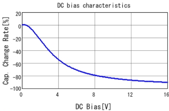
■ GRM188R61C106MAAL C-DC bias capchange, 25.0degC, AC1V
