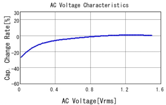
■ GRM188R61C106MAAL C-AC Voltage capchange, DCOV, 25.0d
