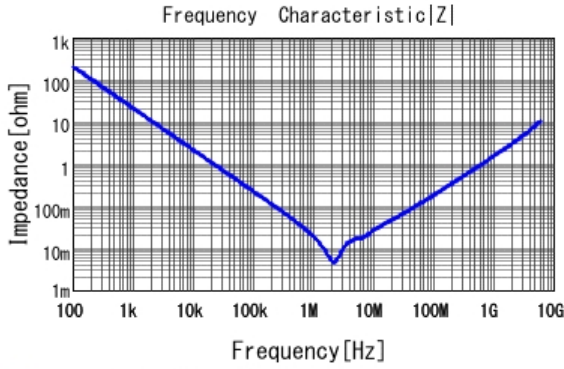
■ GRM188R61C106MAAL |Z| DCOV, 25degC
