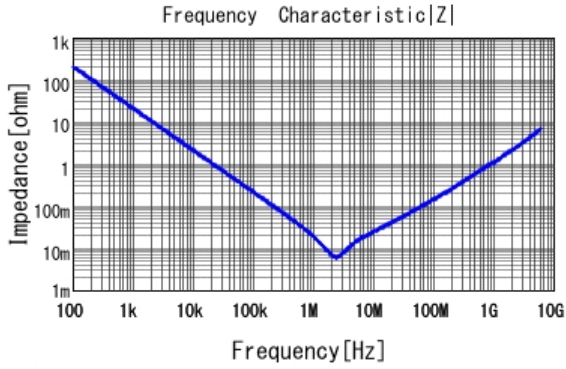
■ GRM155R60G106ME15 |Z| DCOV, 25degC
