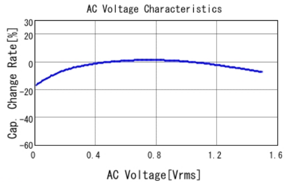
■ GRM155R60G106ME15 C-AC Voltage capchange, DCOV, 25.0d
