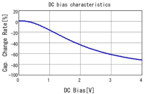
■ GRM155R60G106ME15 C-DC bias capchange, 25.0degC, ACO.
