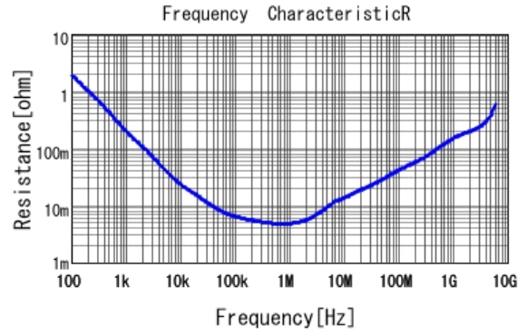
■ GRM155R60G106ME15 R DCOV, 25degC
