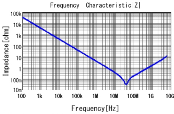
■ GRM155R71C473KA01 |Z| DCOV, 25degC
