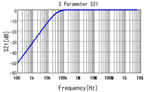
■ GRM155R71C473KA01 S21 DC0V, 25degC
