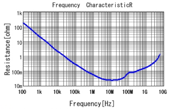
■ GRM155R71C473KA01 R DCOV, 25degC
