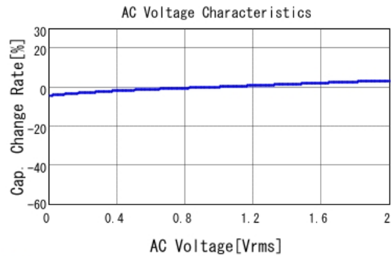
■ GRM155R71C473KA01 C-AC Voltage capchange, DCOV, 25.0d
