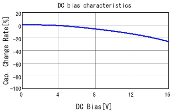
■ GRM155R71C473KA01 C-DC bias capchange, 25.0degC, AC1.
