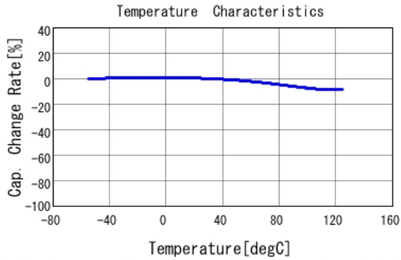
■ GRM155R71C473KA01 C-Temp. capchange, DC0.0V, AC1.0V rm
